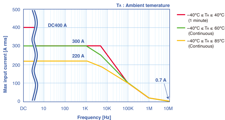
Figure 2. Frequency characteristics
