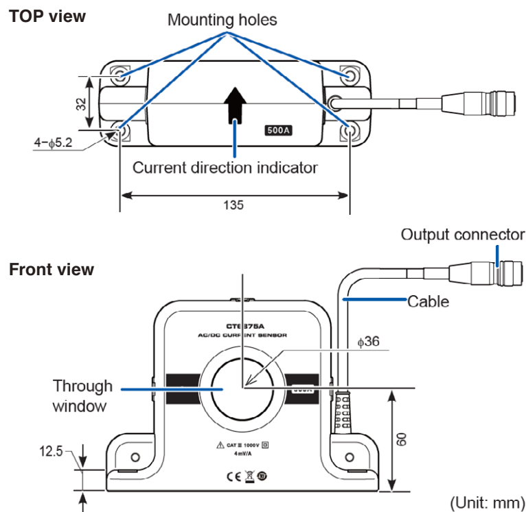
Figure 5. Dimensions
