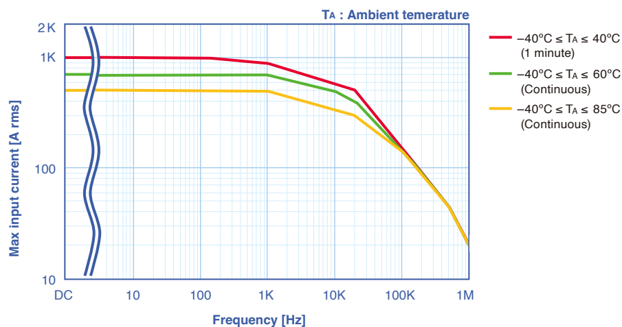
Figure 2. Frequency characteristics
