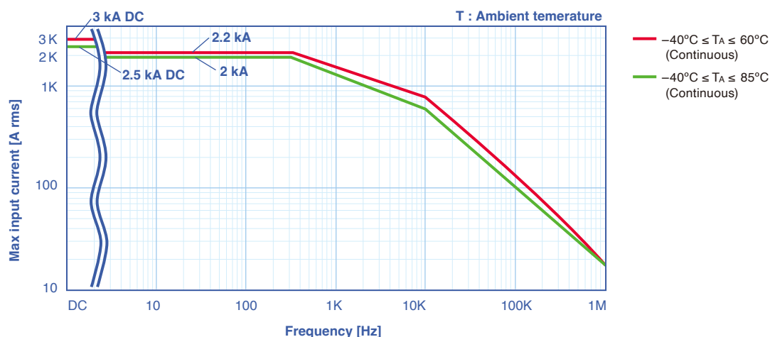
Figure 2. Frequency characteristics
