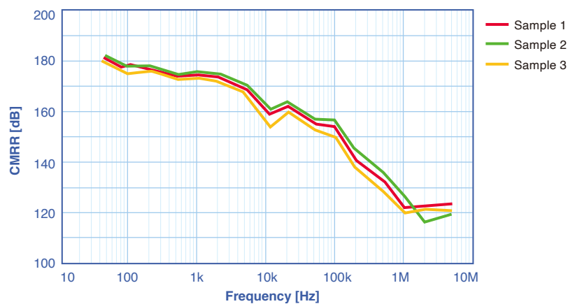
Figure 4. CMRR characteristics
