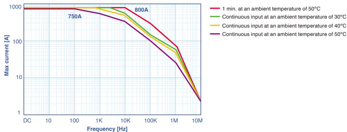
Figure 1. Frequency derating
