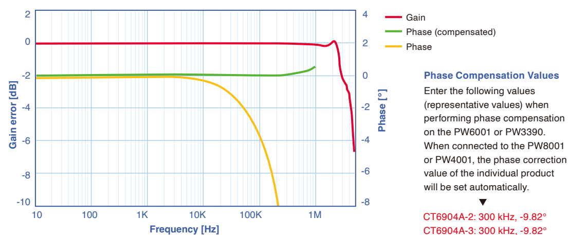
Figure 2. Frequency characteristics
